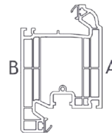
705540 Door Sash Open In
