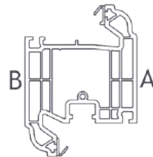
705545 95mm Z Mullion / Slim Door Sash Open In
