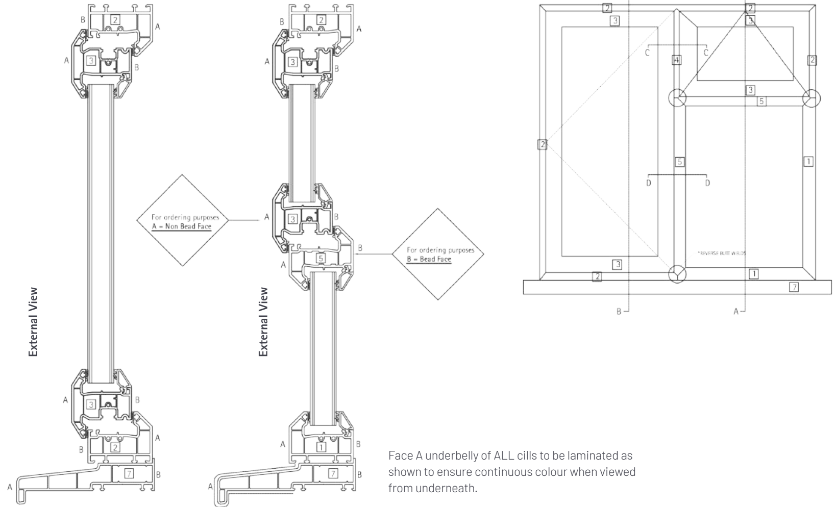
Section B-B
